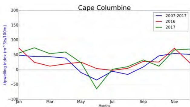
Figure 3: Monthly upwelling strength off Cape Columbine for 2016 and 2017 compared with the 2007-2017 average. Upwelling was stronger than usual during November 2016, and unusually weak in October 2017, with pronounced downwelling in June 2017.
