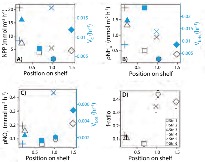
Figure 14: A) NPP and the specific carbon fixation rate ( V_c ), B) pNH_4^+ and the specific NH_4^+ uptake rate ( V_{NH_4} ), C) pNO_3^- and the specific NO_3^- uptake rate ( V_{NO_3} ) and D) the f -ratio (an indication of the strength of the biological pump) at the PP IEP stations. Open black symbols indicate the transport rates (primary y-axis) and solid blue symbols show the specific uptake rates (secondary y-axis). Shelf position was calculated by dividing the distance of each station from shore by the width of the continental shelf at the station latitude; higher shelf positions indicate stations further offshore.
