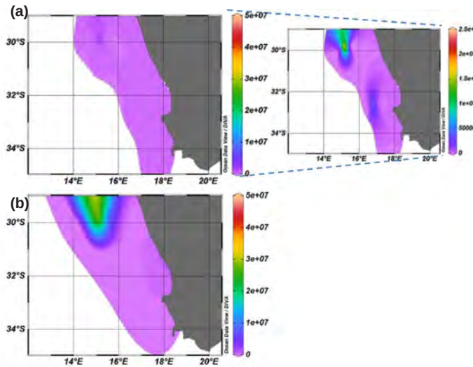
Figure 12: Total phytoplankton abundance (no. m -3 ) during late autumn (May 2016) for (a) the surface, with enhanced scale to the right, and (b) F_{max} (area of the ocean with the highest amount of fluorescence, a proxy of phytoplankton biomass)
