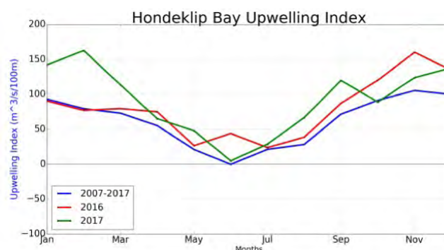
Figure 2: Monthly upwelling strength in Hondeklip Bay for 2016 and 2017 compared with the 2007-2017 average. A maximum well above the long-term mean is observed from October 2016 to March 2017.
