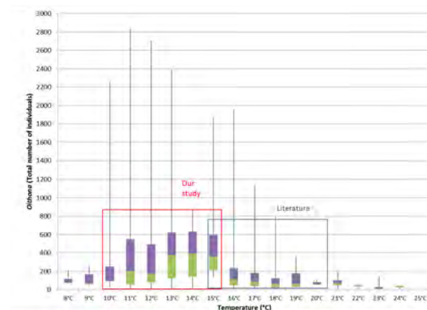
Figure 17: Boxplot showing the abundance of Oithona vs sea surface temperature (SST) with the red box showing the optimal range of Oithona off the west coast of South Africa and the blue box showing the optimal range of Oithona (from the literature).
