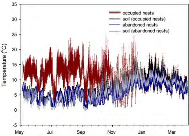
Figure 3: Temperatures in occupied nests and surrounding habitats
