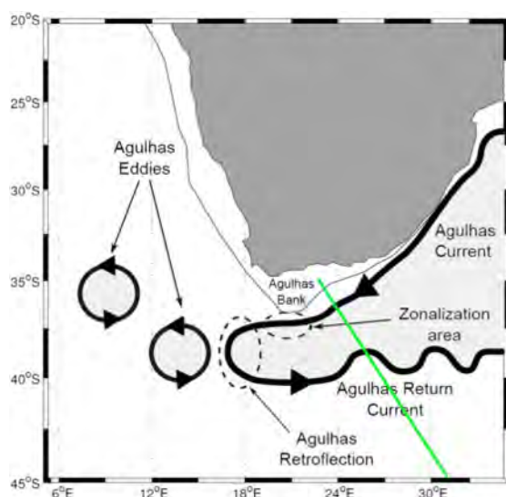
Figure 1: Schematic of the ocean circulation to the south of Africa, showing the Agulhas Current, Agulhas Retroflection and Agulhas Return Current (from Arruda et al. 2014). The approximate cruise track during annual relief voyages to Marion Island is shown in green.
