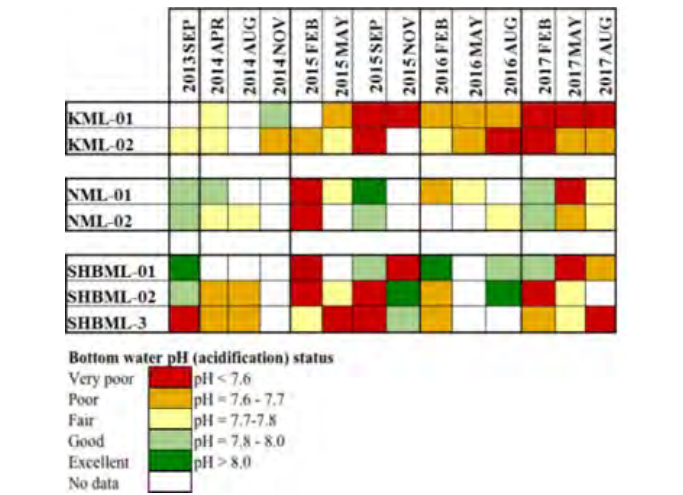
Figure 5: Annual variability in pH of inshore bottom water
