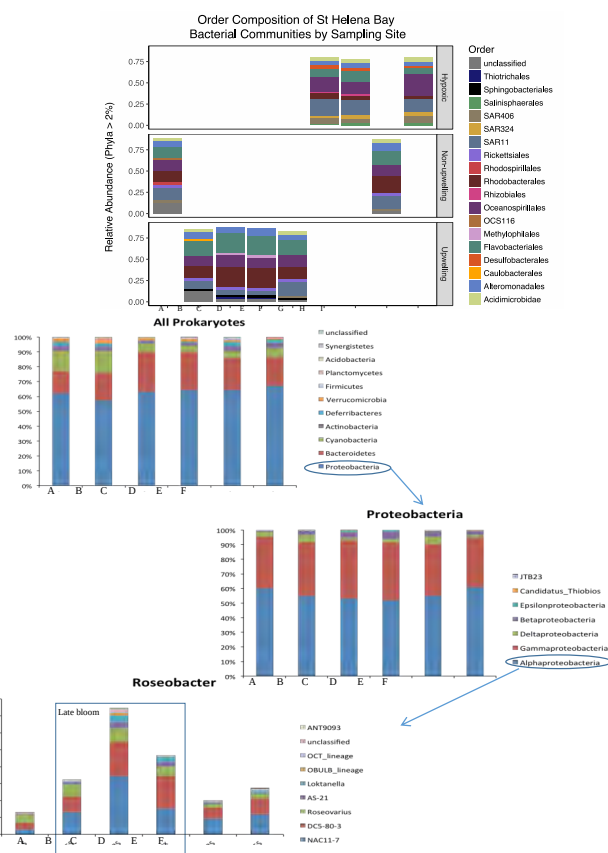
Figure 10: Results from genetic analysis of prokaryotes: samples for May: A. station 7 surface, B. station 5 surface, C. station 3 surface, D. station 3 F_{max} ; samples for September: E. Station 13 surface, F. station 5 surface, G. station 13 bottom, H. station 13 bottom, I. station 5 bottom.
