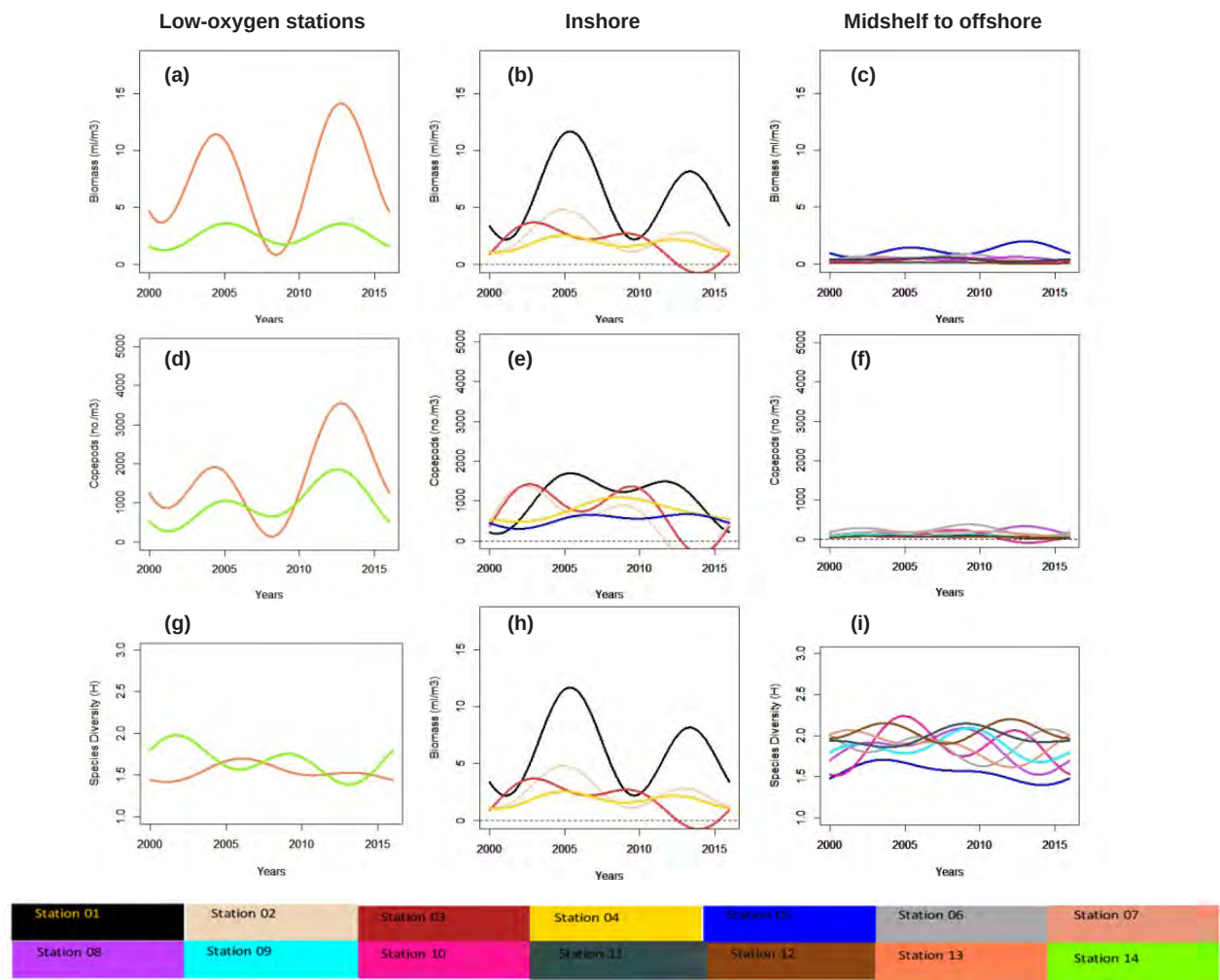
Figure 15: Functional data analysis was used to determine the following patterns: biomass of mesozooplankton along SHBML at (a) low-oxygen stations 13 and 14, (b) inshore stations 1 – 4, (c) midshelf to offshore stations 5 – 12; copepod abundance along SHBML at (d) low-oxygen stations 13 and 14, (e) inshore stations 1 – 4, (f) midshelf to offshore stations 5 – 12; species diversity of mesozooplankton along SHBML at (g) low-oxygen stations 13 and 14, (h) inshore stations 1 – 4 and (i) midshelf to offshore stations 5 – 12. See Fig. 8 for map with station numbering.
